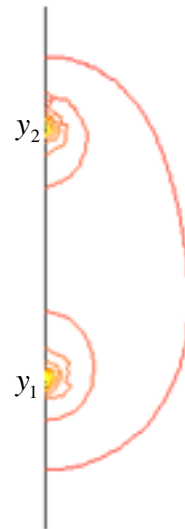
b. Contours of total heat flux magnitude
