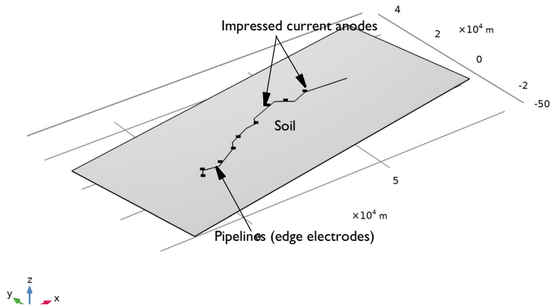
Figure 1: The model geometry consists of three pipelines, nine impressed current anodes, and two soil layers.
